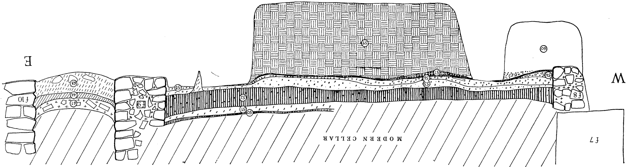
Fig. 2 Sections across Aldersgate Street and Medieval Cellar
